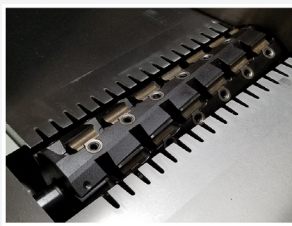
Spiral insert knife cutterhead with 30 x 12 x 1.5 mm two-sided insert knives
